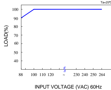
SPS- 100-xx series without PFC choke
