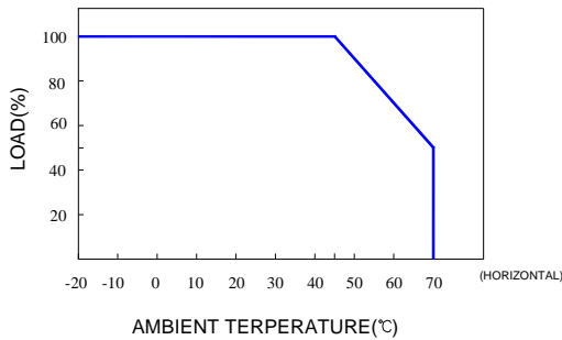
SPS- 100-xx series without PFC choke
