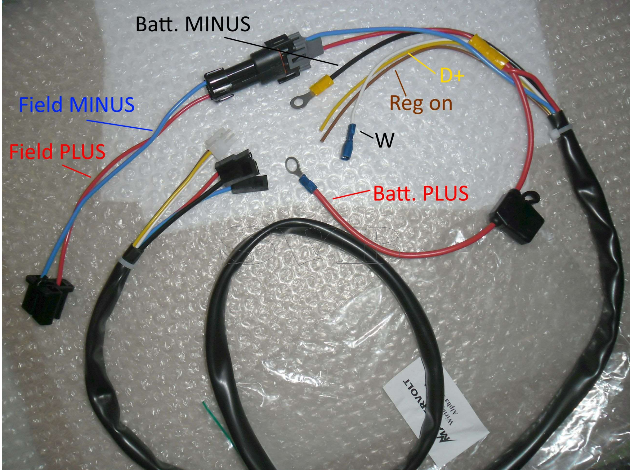
20174 MASTERVOLT alpha pro wiring harness
