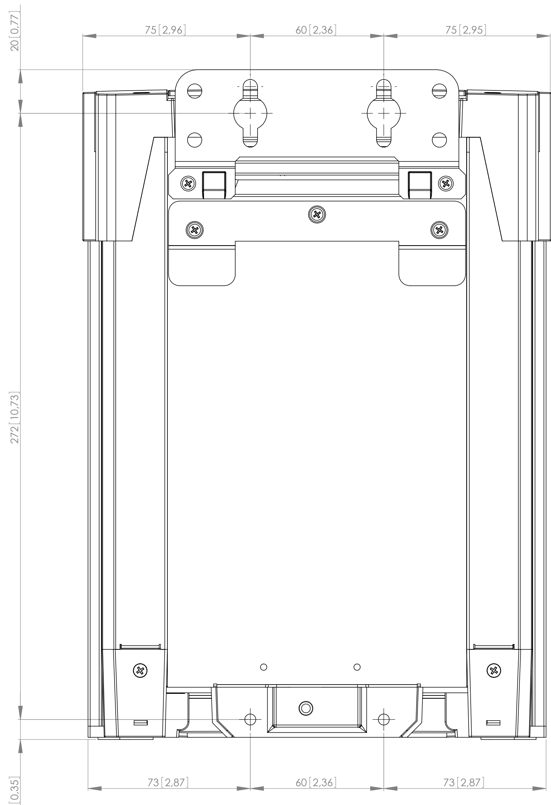
Mounting bracket in 'up' position
